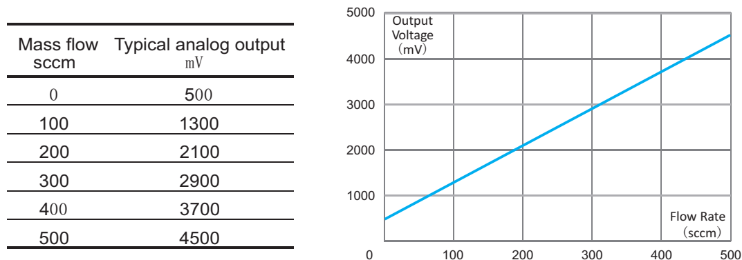
Figure 1.1: The typical analog output curve of FS8001.
