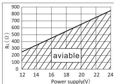
Figure 6-4. 4~20mA External Connection
